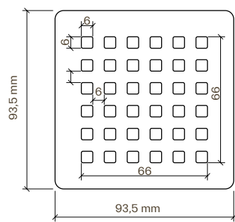
Grate top view
