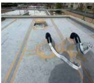
Waterproofing of walkable flat roofs with ECODRY120 . RESIDENTIAL SINGLE-FAMILY HOMES. Montevideo. Uruguay.
