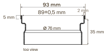
D/D_drainage base
