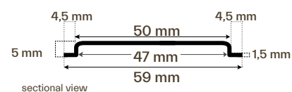
B/B_drainage base
