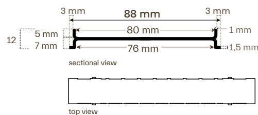
D/D_drainage base
