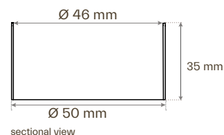
B/B_drainage base
