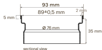
B/B_drainage base
