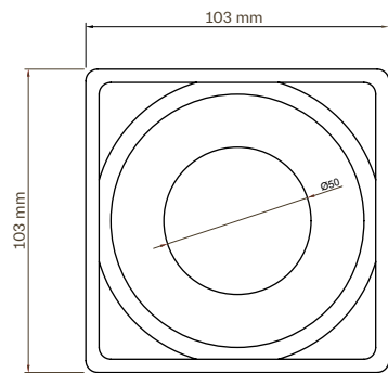
Top view lifting frame
